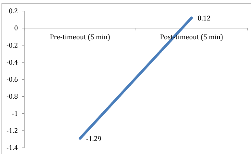
Fig. (2). Cumulative effects of timeouts on game score.
