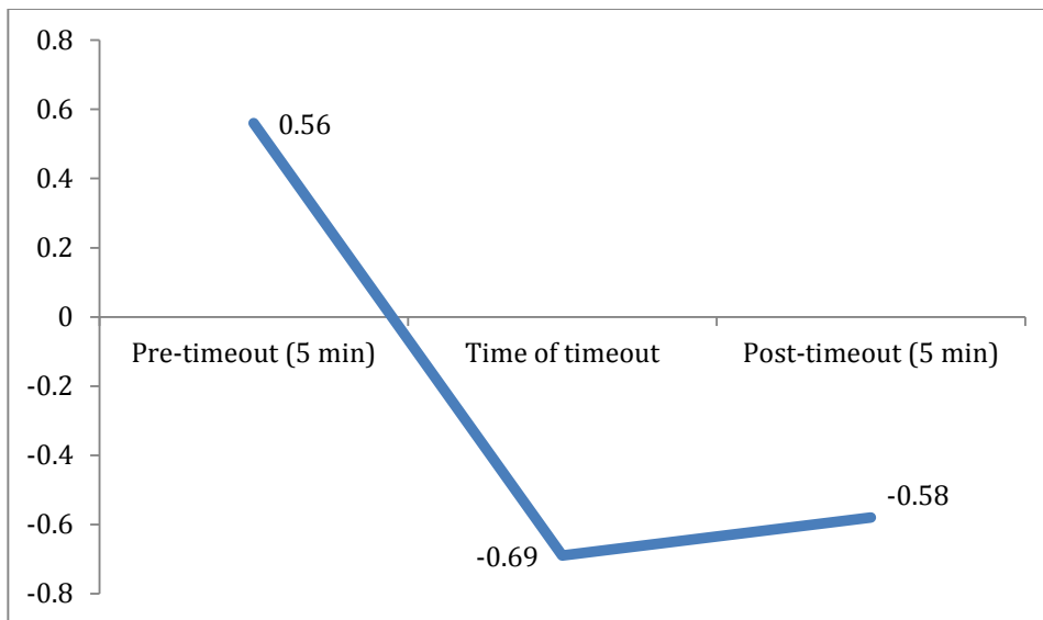
Fig. (1). The effects of timeouts on game score.
